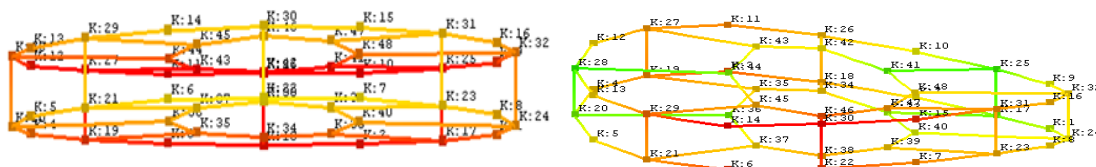
Fig. 4: Comparison of the mode I of the new wheel on the left side (302.775 Hz, 3.65%) with the mode I of the worn wheel on the right side (300.728 Hz, 0.16%)
